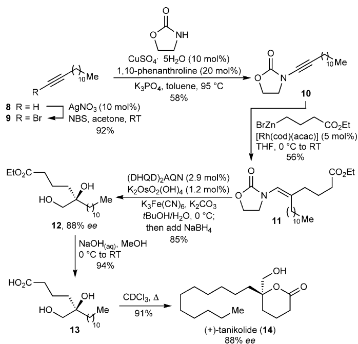
Scheme 4. Total synthesis of (+)-tanikolide ( 14 ). cod = cycloocta-1,5-diene, NBS = N-bromosuccinimide.
