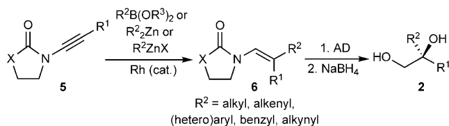
Scheme 2. Asymmetric dihydroxylation of enamides prepared by rhodium-catalyzed carbometalation of ynamides.
