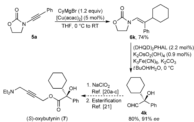
Scheme 3. Synthesis of \alpha -hydroxyaldehyde 4k , a precursor to (S)-oxybutynin ( 7 ). THF = tetrahydrofuran.
